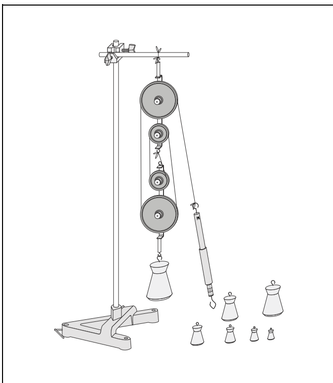
Fig. 4 Setup with pulley block
